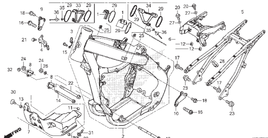
C-39 Chassi
